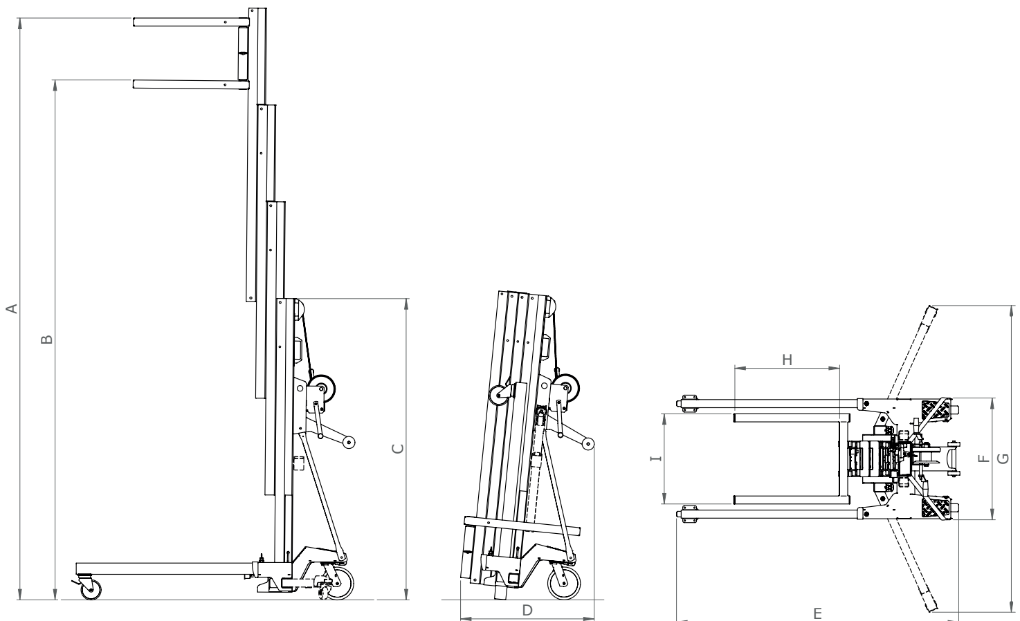
Illustration Materiallift
